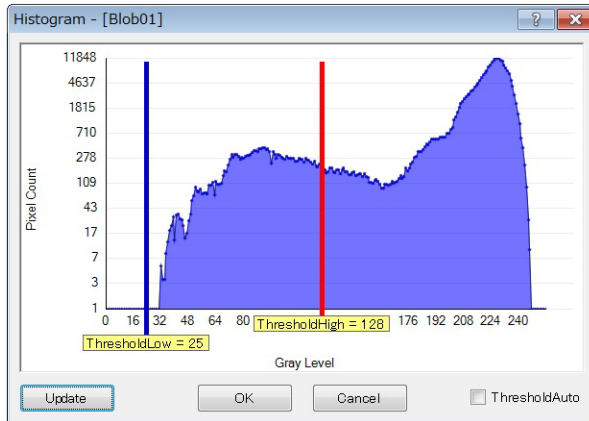
Histogram of Rings Image with better Threshold Settings
