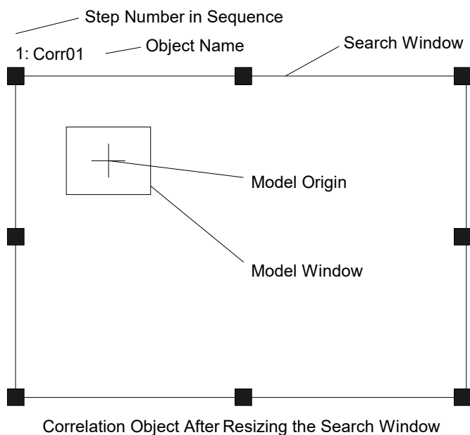
Search Window shown after resizing
