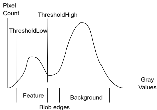
Setting the threshold values using a histogram
